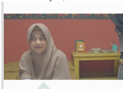
Gambar 4.3 Screenshot Rara
