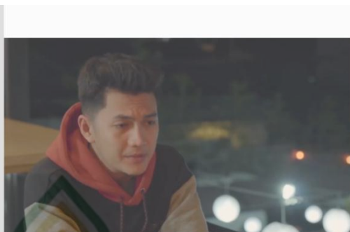
Gambar 4.7 Screenshot Dewa
